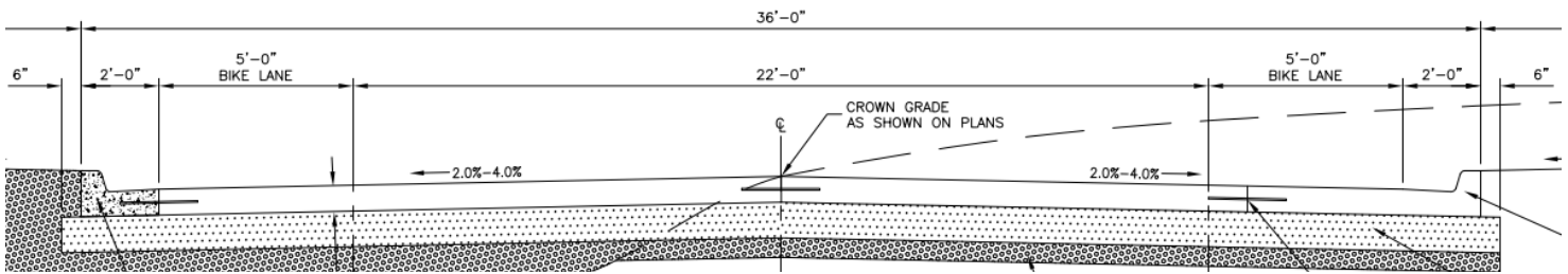
Typical Section - 36' Street (Collector)
