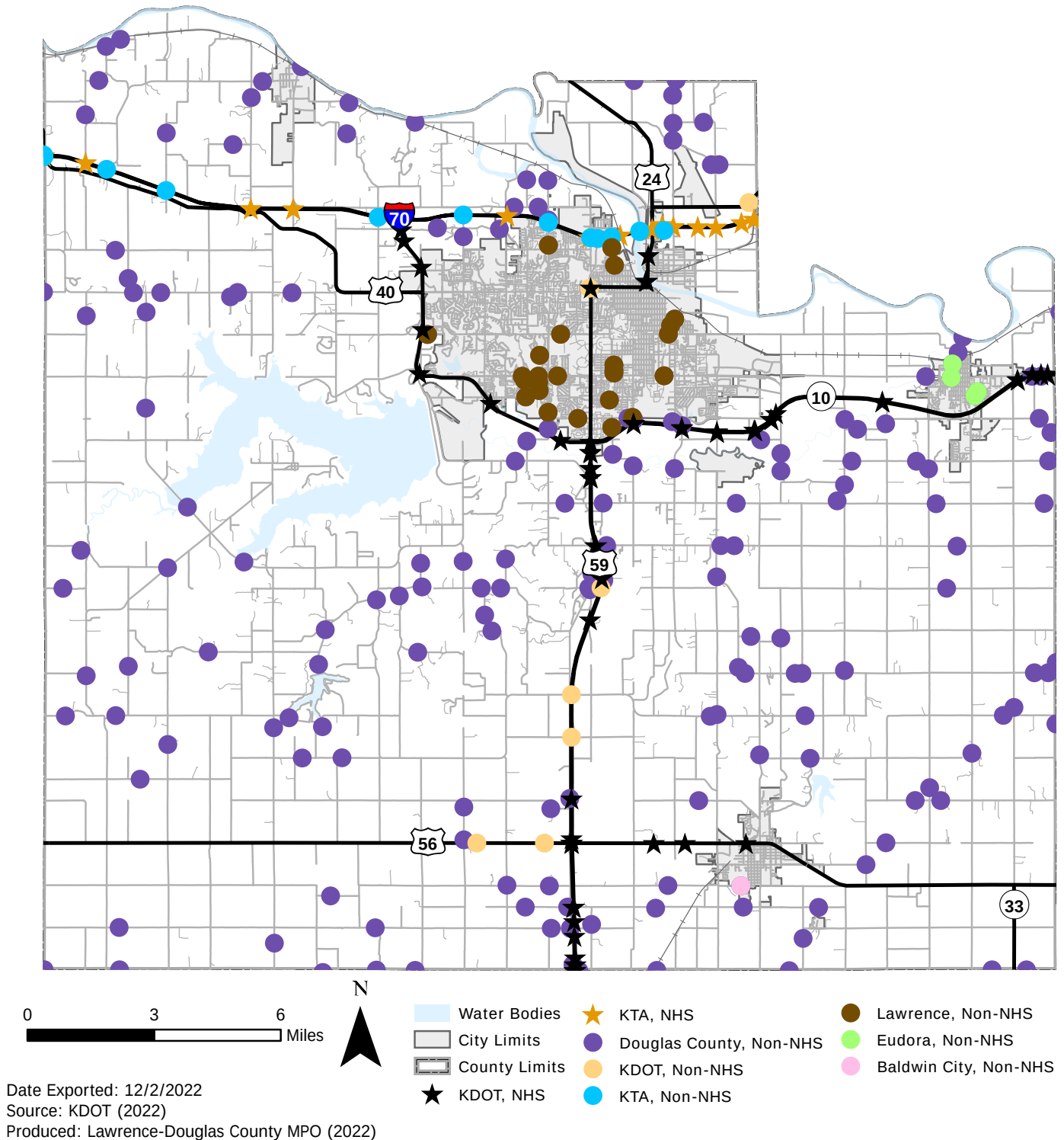
Figure 2.28: National Highway System (NHS) and Non-NHS Bridge
