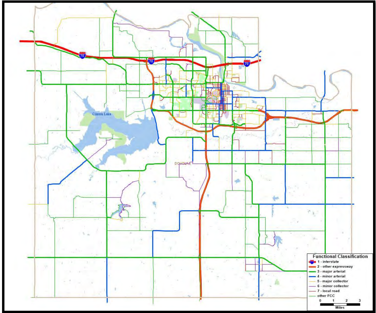
Modeled road network showing functional classification—Douglas County
